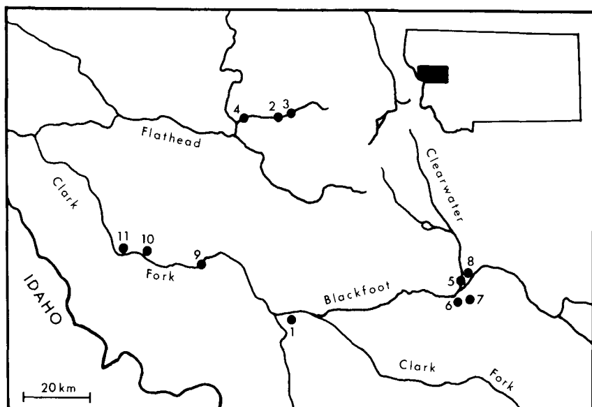
FIG. 1. Distribution of collecting sites in western Montana.
