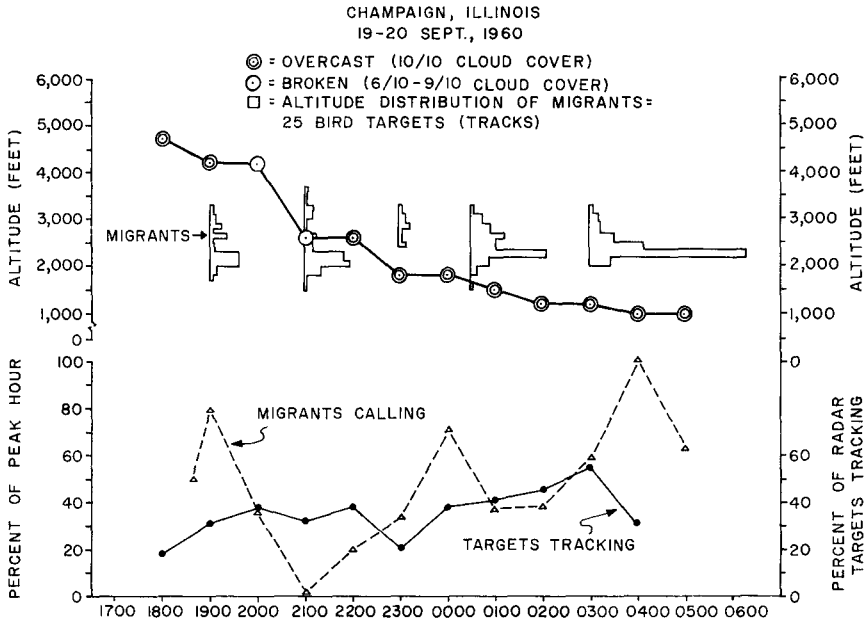
FIG. 3. Hour-to-hour variation in patterns of calling and tracking by migrants on an overcast night. Circle symbols and heavy line show altitude of cloud cover. Open square symbols show altitude and number of migrants.
