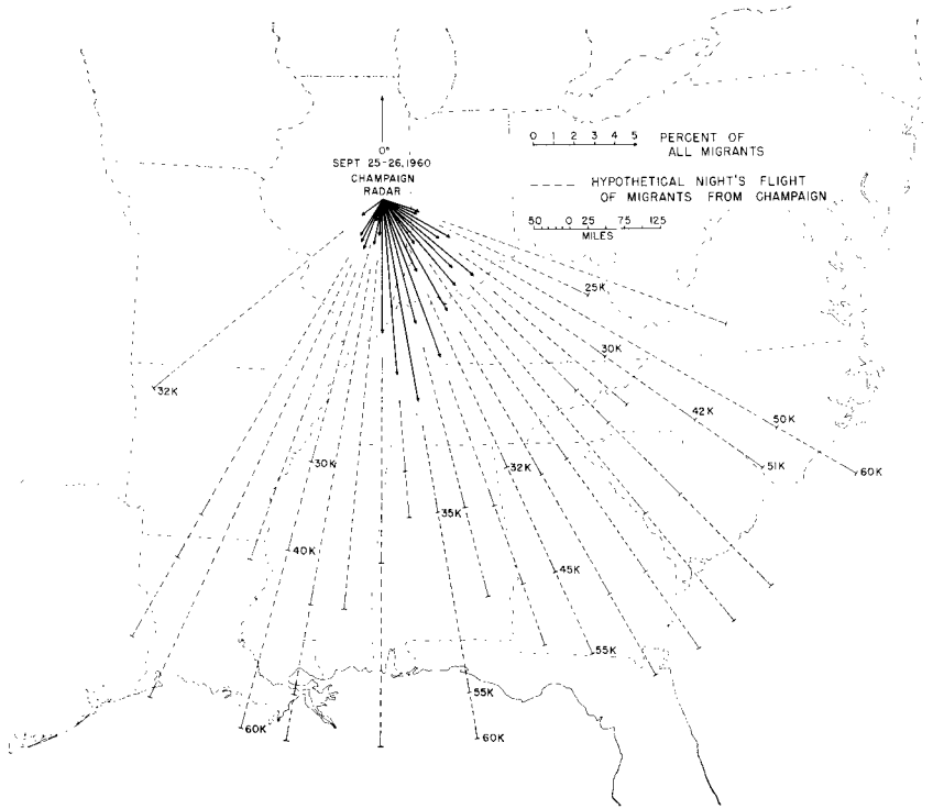
FIG. 7. Flight directions of migrants recorded by radar on a typical clear Fall night. Heavy arrows show the per cent of migrants on a given 5-degree track. Dash lines extend the radar tracks through a full night's migration, the extrapolation based on each track direction, its speed in knots (K), and the temporal pattern observed at Champaign.
