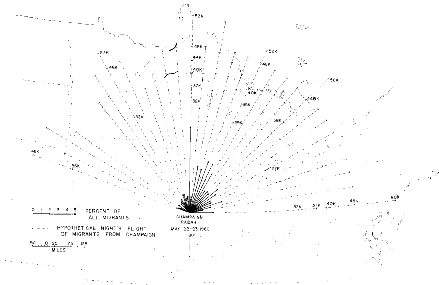
FIG. 6. Flight directions of migrants recorded by radar on a typical clear Spring night. Heavy arrows show the per cent of migrants on a given 5-degree track. Dash lines extend the radar tracks through a full night's migration, the extrapolation based on each track direction, its speed in knots (K), and the temporal pattern observed at Champaign.
