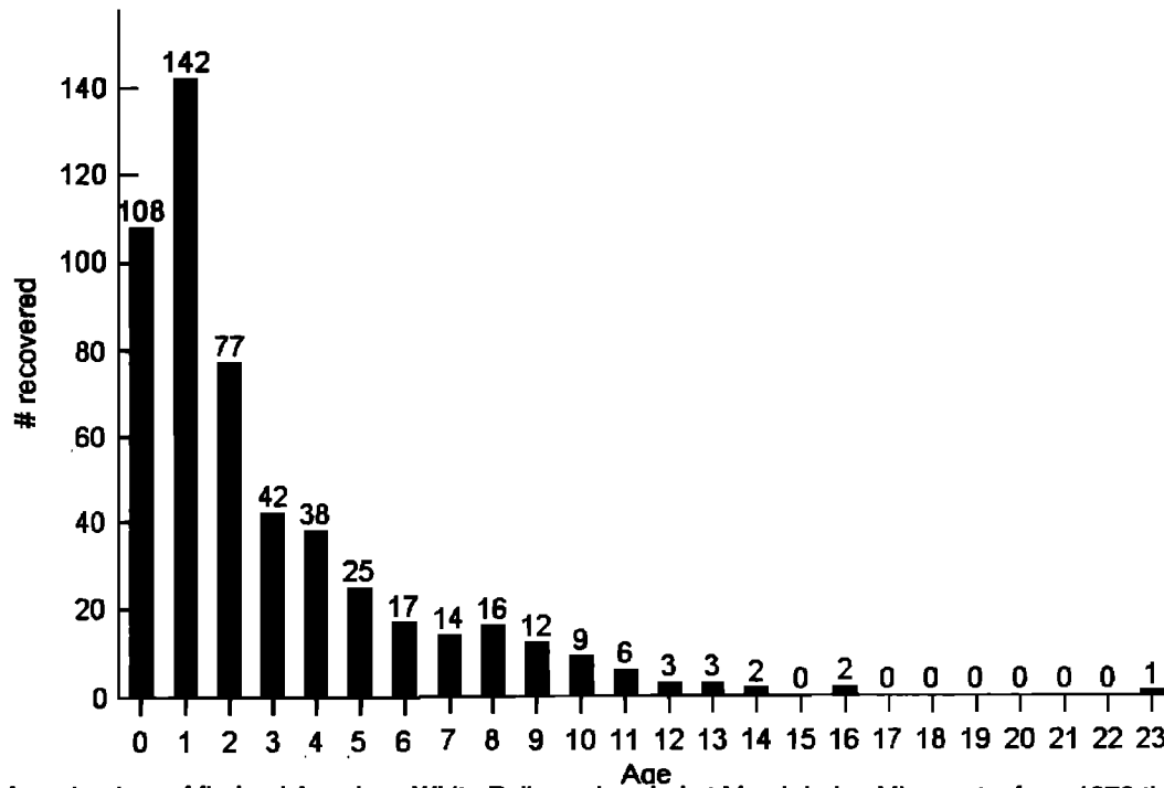
Fig. 2. Age structure of fledged American White Pelicans banded at Marsh Lake, Minnesota, from 1972 through 1998.
