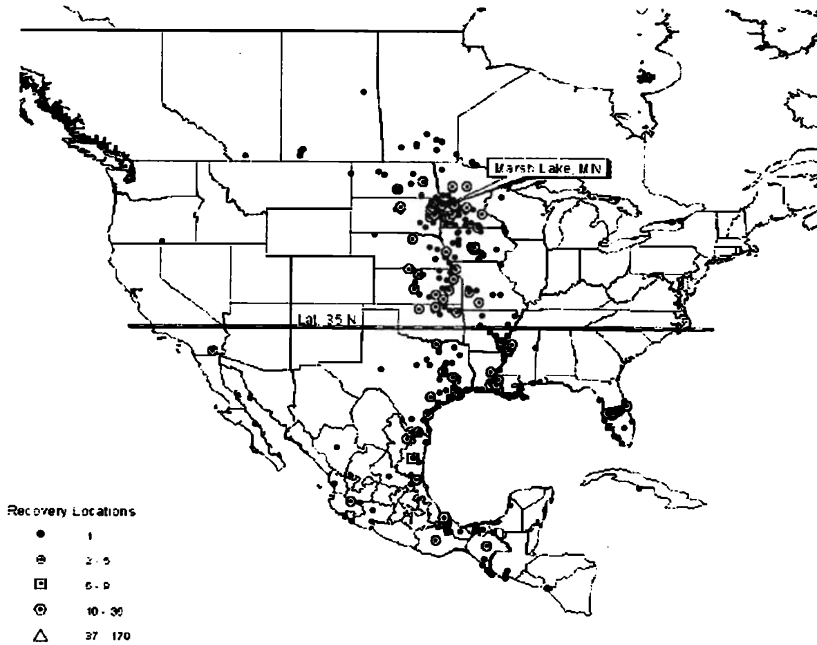
Fig. 1. Recovery locations of American White Pelicans banded as fledglings at Marsh Lake, Minnesota, from 1972 through 1998.
