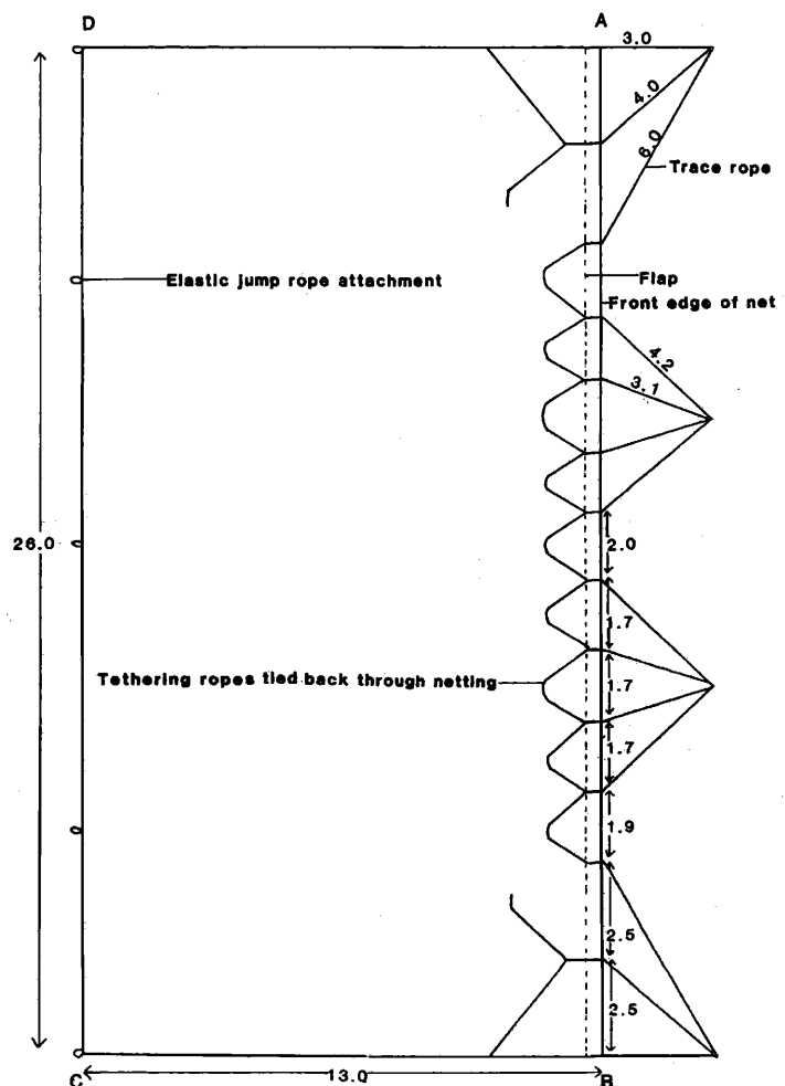
Figure 1. The design of a full-sized net. All measurements are in metres.
