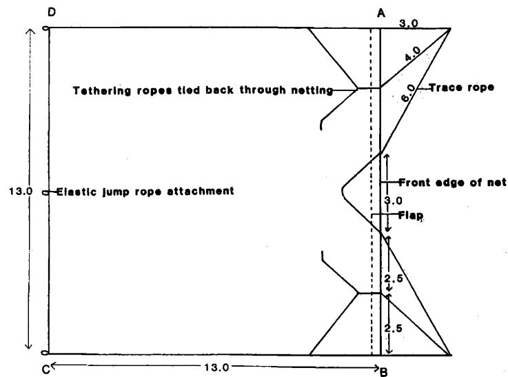
Figure 2. The design of a half-sized net. All measurements are in metres.
