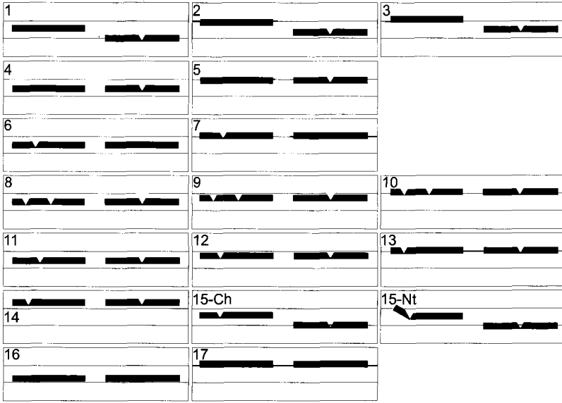
FIG. 2. Diagrams (see Fig. 1) of songs representing 17 groups from our cluster analysis (see Table 1), showing the relative uniformity of Black-capped Chickadee songs throughout mainland North America (clusters 1 to 3) and the great diversity of songs on the offshore islands of Massachusetts (clusters 4 to 17). Frequency markers are 2 to 5 kHz, and the duration of each diagram is about one second, as in Figure 1; frequency and temporal characteristics for each diagram are based on average values for each cluster. Clusters 1 to 3 are low-, medium-, and high-frequency two-tone hey-sweetie songs (i.e. fee-bee-ee) from throughout North America; clusters 4 and 5 the low- and high-frequency monotonal hey-sweetie songs, mostly from Chappaquiddick; clusters 6 and 7 the low- and high-frequency sweetie-hey songs exclusively from Martha's Vineyard; clusters 8 to 10 the low-, medium-, and high-frequency sosweetie-sweetie songs found mostly on eastern Martha's Vineyard; clusters 11 to 14 the low to high monotonal sweetie-sweetie songs (Martha's Vineyard and Chappaquiddick); cluster 15 is the two-tone sweetie-sweetie song (Chappaquiddick and Nantucket); and clusters 16 and 17 the monotonal hey-hey, found mostly on Nantucket. We illustrate two diagrams for cluster 15 because songs from Chappaquiddick (Ch) and Nantucket (Nt) were separable by our ears and by sonagrams, even though they were combined by the cluster analysis.
