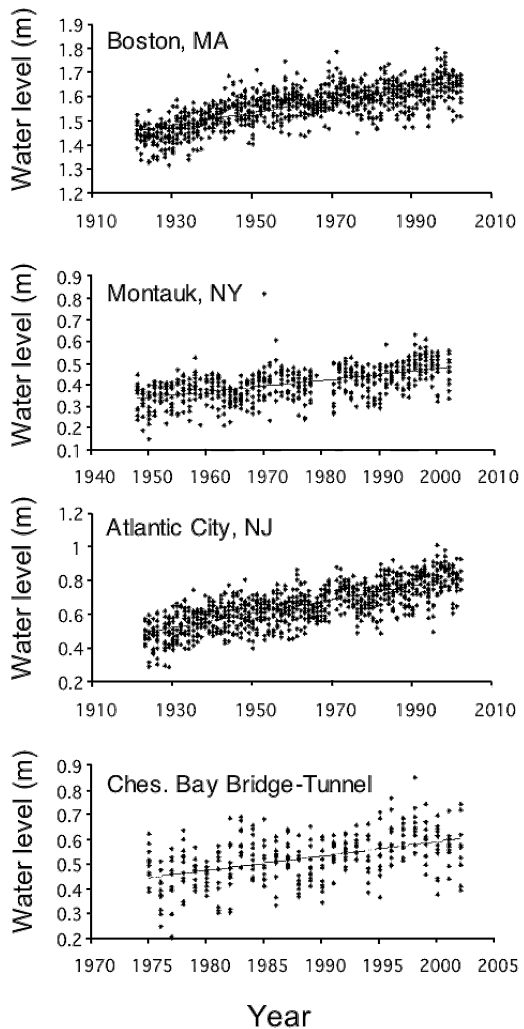
FIGURE 4. Comparison of relative sea-level rise rates along the Atlantic Coast based on monthly mean tide heights (datum mean low low water). Raw data obtained from National Oceanic and Atmospheric Administration's (NOAA) National Ocean Service (< http://www.co-ops.nos.noaa.gov/ > (31 July 2006)). Annual RSLR rates, regression equations, r^2 values, and P-values are: Boston: rate = 0.26 cm/yr, y = -3.48 + 0.00257x , r^2 = 0.55 , P < 0.01 ; Montauk: 0.26 cm/yr, y = -4.76 + 0.0026x , r^2 = 0.31 , P < 0.01 ; Atlantic City: 0.41 cm/yr, y = -7.4 + 0.0041x , r^2 = 0.58 , P < 0.01 ; Chesapeake Bay Bridge-Tunnel: 0.59 cm/yr, y = -11.2 + 0.0059x , r^2 = 0.23 , P < 0.01 .
