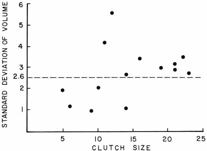
FIGURE 3. Comparison of standard deviation of egg volume with clutch size in 14 sets of Wood Duck eggs. See text for explanation.
