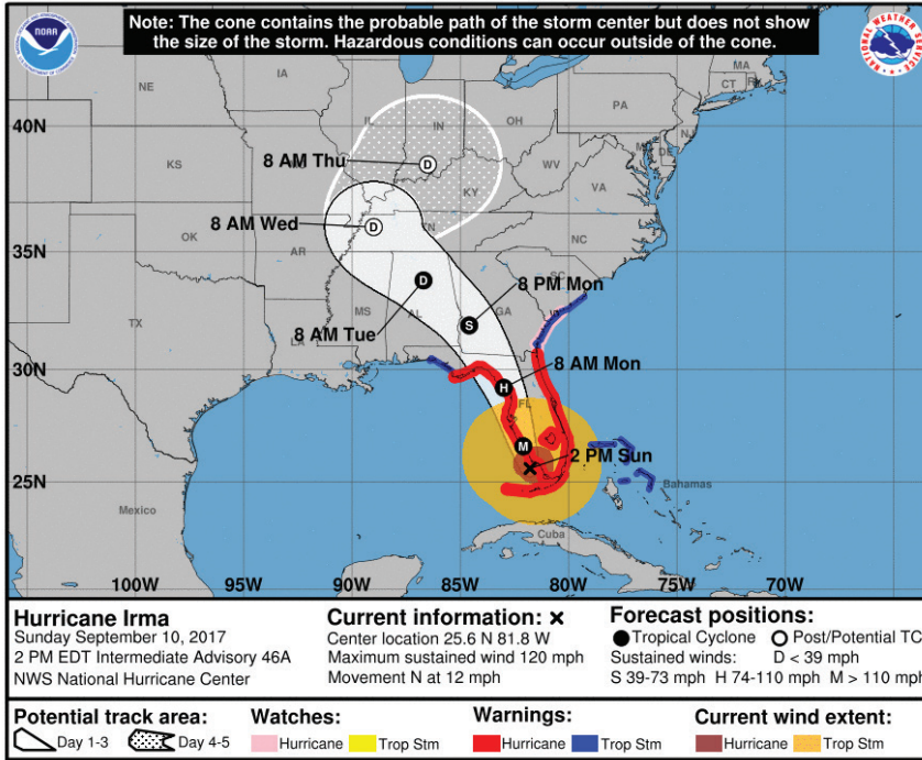
Figure 1. The predicted track of Hurricane Irma in 2017, issued for the public by the National Oceanic and Atmospheric Administration and the National Weather Service.
